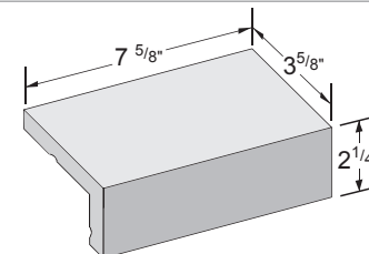
Modular Edge Cap 2 1/4" x 3 5/8" x 7 5/8" (Excludes 710 Charcoal)
