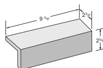
King Edge Cap 2 5/8" x 2 3/4" x 9 5/8"
