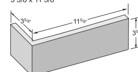
Utility Corner 3 5/8" x 3 5/8" x 11 5/8"
