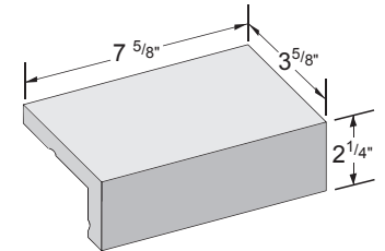
Modular Edge Cap 2 1/4" x 3 5/8" x 7 5/8"
